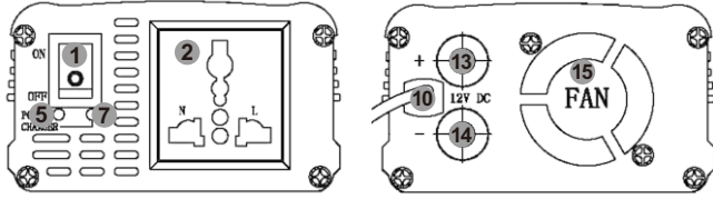
BEU500L/600L/800L/1000L UPS逆变器面板
