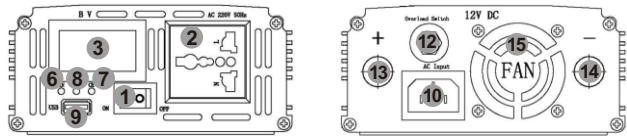
BEU1200L/1500L UPS逆变器面板
